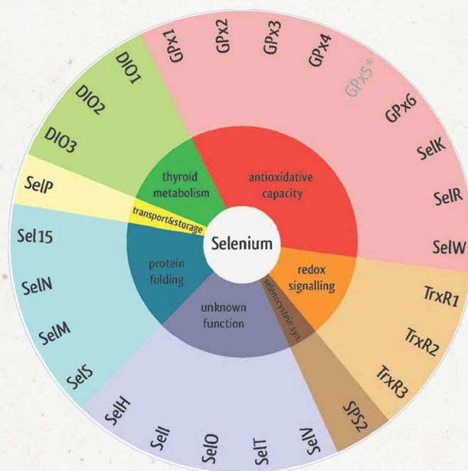
Figure 2: Classes of selenoproteins and their putative functions (8).
